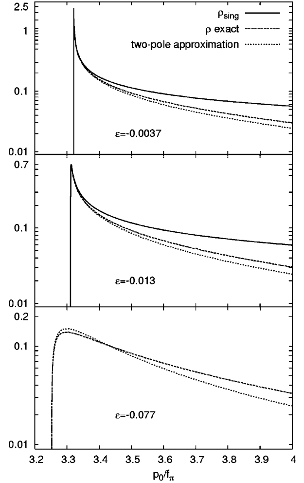
FIG. 2. The spectral function \rho(p_0, \epsilon) f_\pi^2 in various approximations as a function of p_0 at different reduced temperatures \epsilon , and |\mathbf{p}|=0 .
